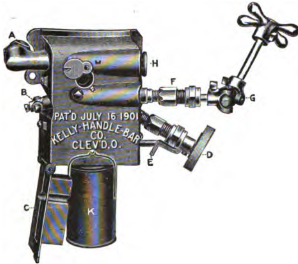
FIG. 222.—The Starter Box and Control Valve of the Kelly Burner. A , union joint to supply pipe; B , gas orifice leading direct to the main burner; C , drop drip cup and bottom of case; D , sub-flame valve; E , check on valve to prevent turning by vibrations of travel; F , packing nut on the main fire valve; G , knuckle joint to carry rod to seat; H , opening to screw on the diaphragm regulator; K , the alcohol lamp hung in position to start vaporizing and fire the burner.
